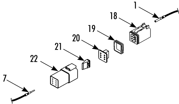
6-pin Connector
