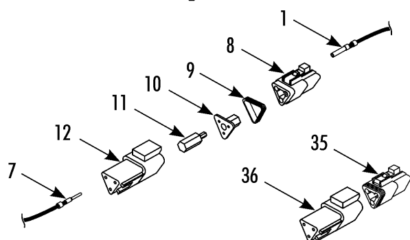
3-pin Connector
