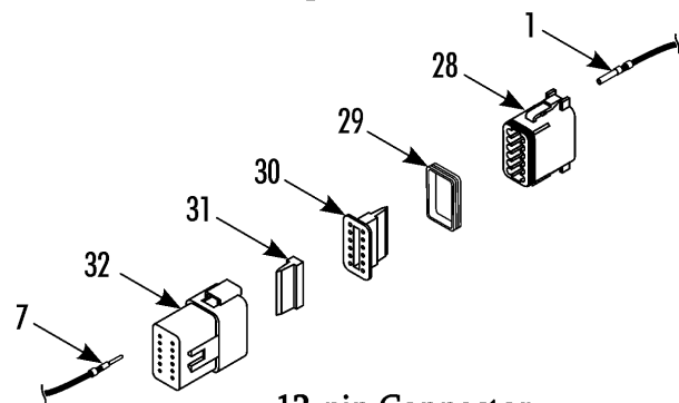
12-pin Connector
