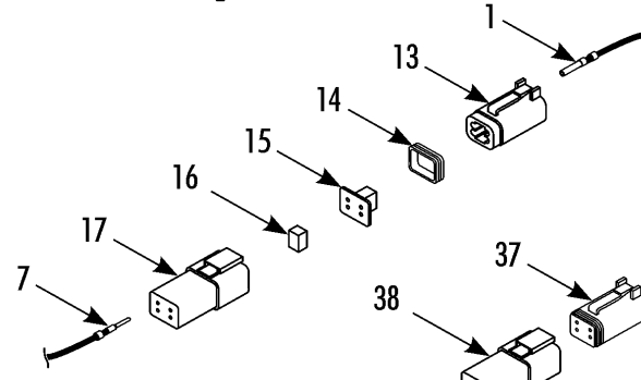
4-pin Connector
