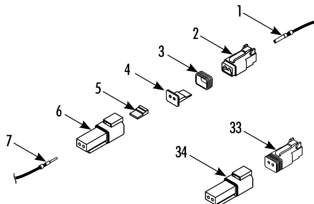
2-pin Connector
