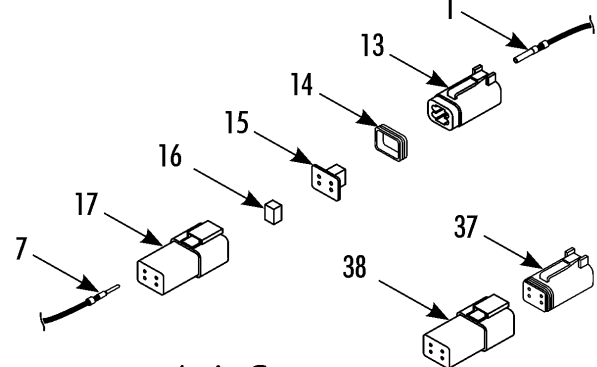
4-pin Connector
