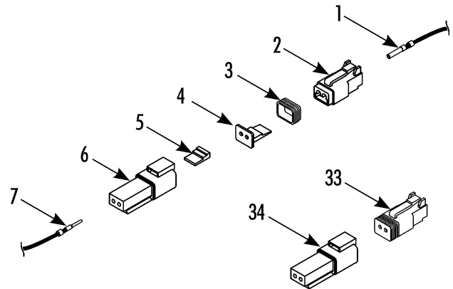
2-pin Connector
