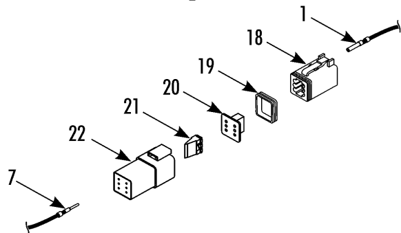
6-pin Connector
