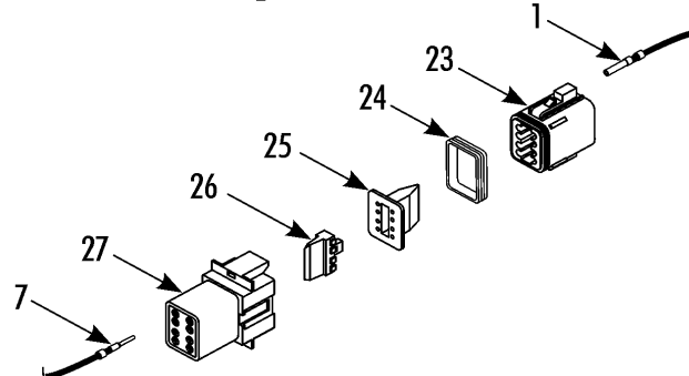
8-pin Connector
